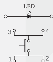
(SPST) Contact Configuration
